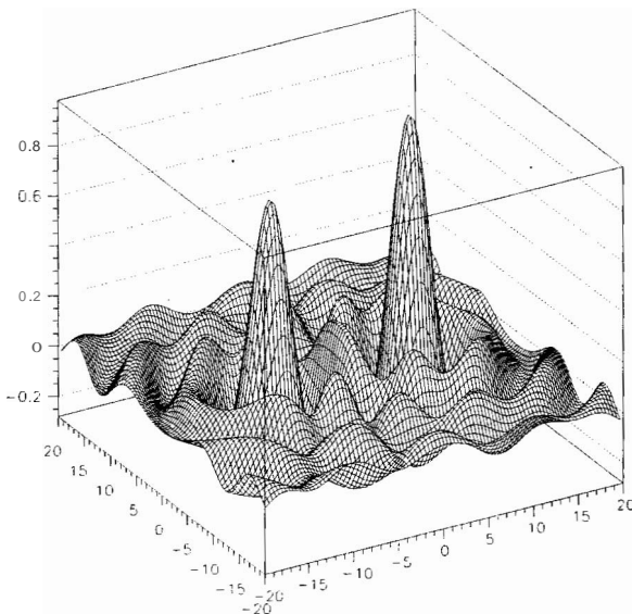
Fig. 1. Sample Fitness Landscape (© Karel Soustruznik, reproduced by permission)
